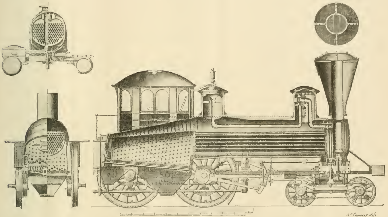
SECTIONAL VIEWS OF JAMES MILHOLLAND'S ANTHRACITE COAL BURNING PASSENGER LOCOMOTIVE "HIAWATHA," ABOUT 1874.
